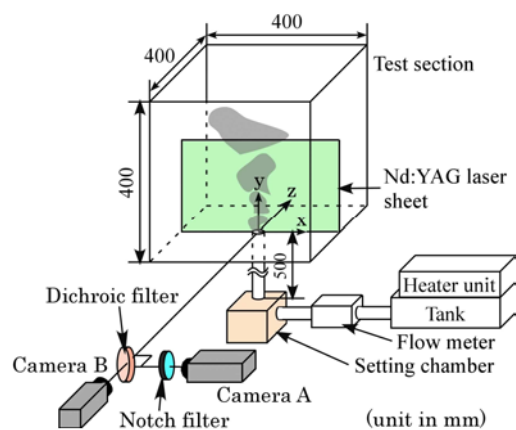
Fig. 1. Experimental setup.
