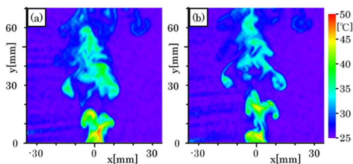
Fig. 4. Instantaneous temperature contours of plume.
